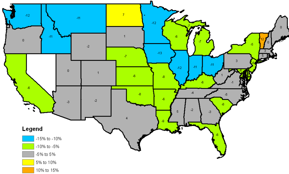
Corn Percent Change in Total Rate
