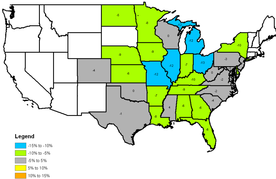
Soybeans Percent Change in Total Rate
